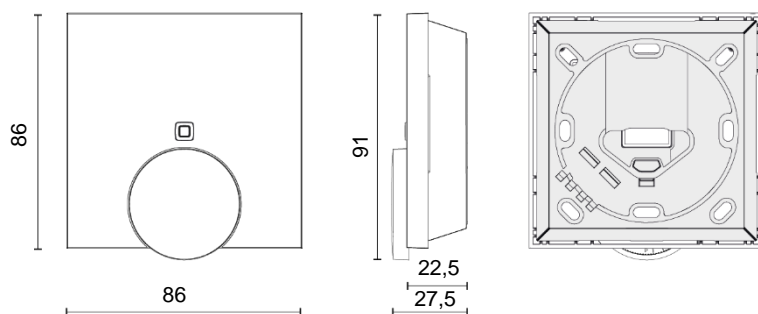
Fig. 1: Dimensions COMFORT IP Room Control Unit Radio Analog (indications in mm)
